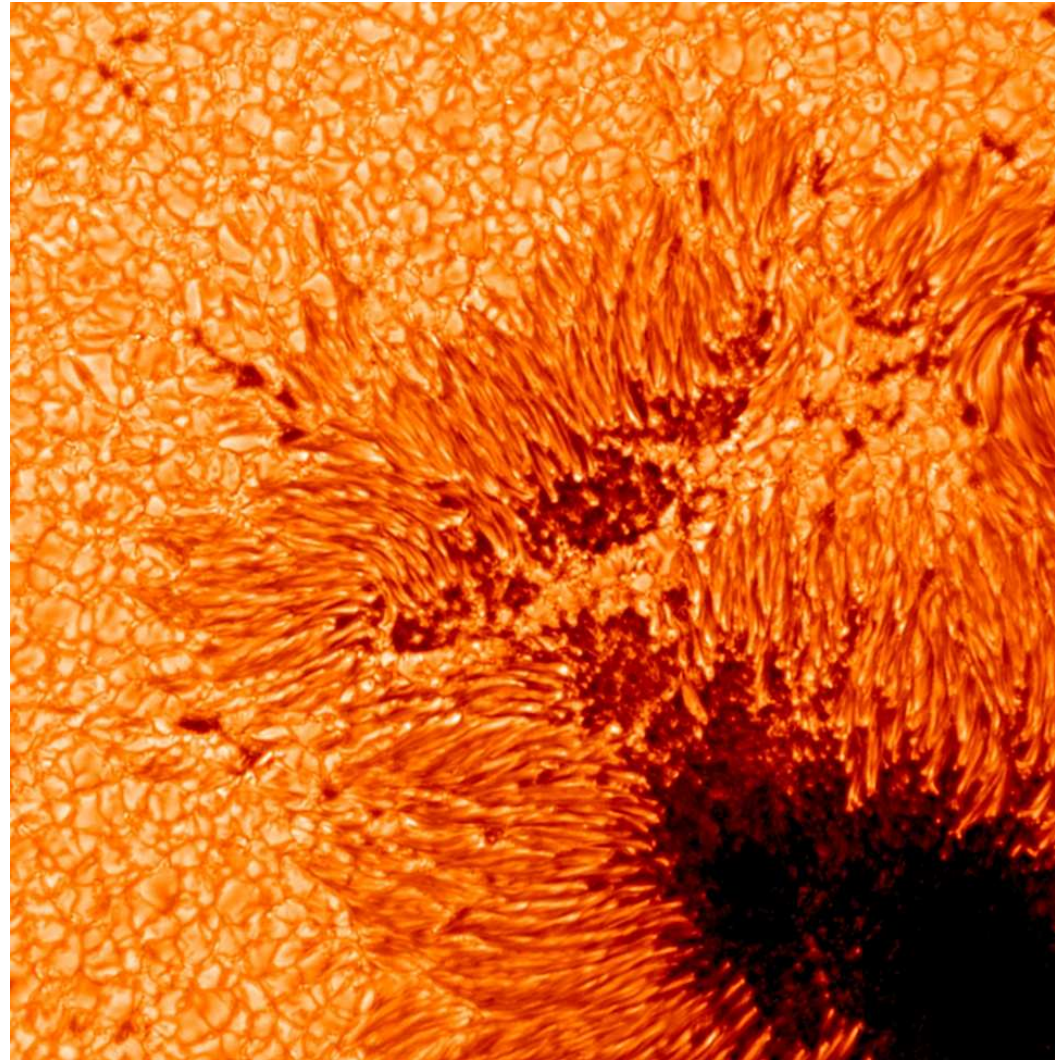
This high-resolution image of active region NOAA 10756 was obtained with the new high-order adaptive optics system at the Big Bear Solar Observatory on May 2nd, 2005. Speckle interferometric techniques were used to restore the image across the entire field-of-view of 55 Mm x 55 Mm.
