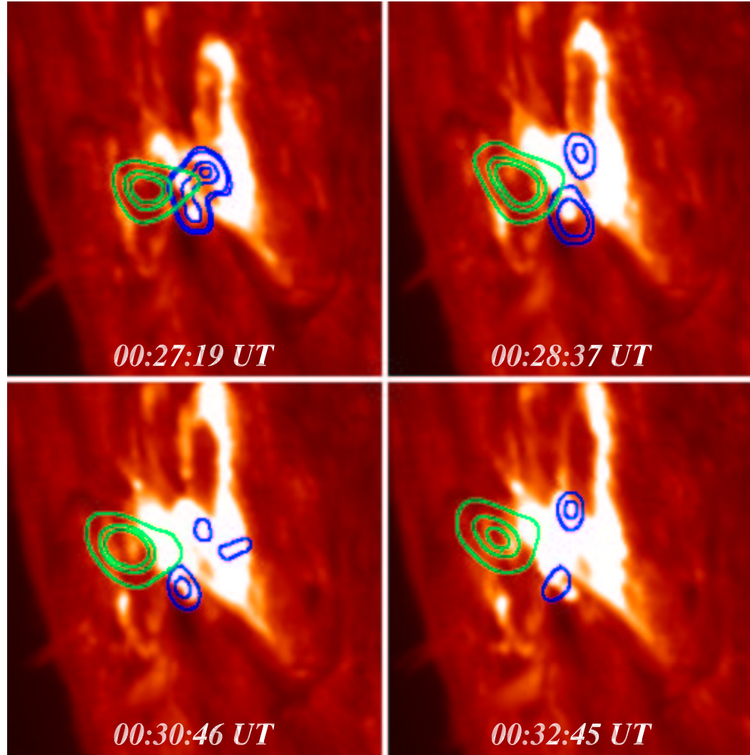
The X4.8 flare on July 23, 2002 was the sole Gamma-Ray flare observed by the Ramaty High Energy Solar Spectroscopic Imager (RHESSI) so far. The flare was observed by Big Bear Solar Observatory (BBSO). The background images are BBSO Halpha filtergrams from full-disk at 4 different times near the peak of the flare. Green contours are the corresponding RHESSI hard X-ray emissions in the energy range of 12 to 20 keV, while the blue contours are for the \gamma -ray energy range between 100 to 150 keV.
