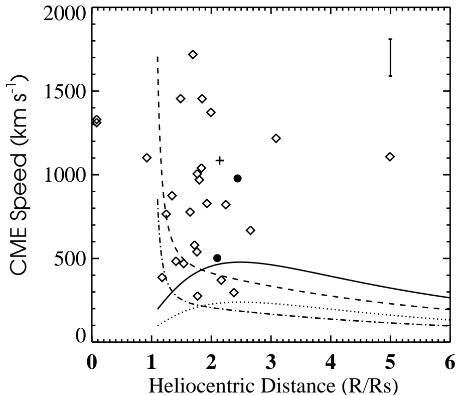
Figure 4. CME speed vs type II formation height extrapolated using the constant speed method. The original locations of two events near the heliocenter, which were estimated from the extrapolations, are -4.4R_{\odot} and -1.6R_{\odot} , respectively. Speeds and heights of the CMEs measured with LASCO C1 and MLSO Mk IV observations are designated by cross and filled circle symbols, respectively. Alfvén speeds are computed using 1\times Newkirk density model (solid line) and 4\times Newkirk model (dotted line) for the quiet magnetic field model. The speeds are also estimated using 1\times Newkirk model (dashed line) and 4\times Newkirk model (dash dot line) for the active region magnetic field model. The error bar in right upper corner indicates the mean error ( 110 \text{ km s}^{-1} ) of extrapolation estimated from three events in Table 3.
