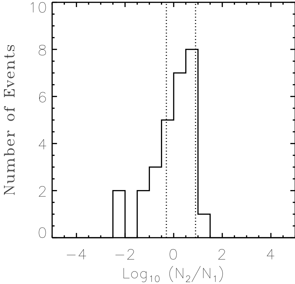
Figure 7. Distribution of the density multiplier for which the type II speed is consistent with the CME speed. Left vertical dotted line denotes the density of low density region (0.5-fold Newkirk model) and right vertical line indicates that of coronal streamer (8-fold Newkirk model).
