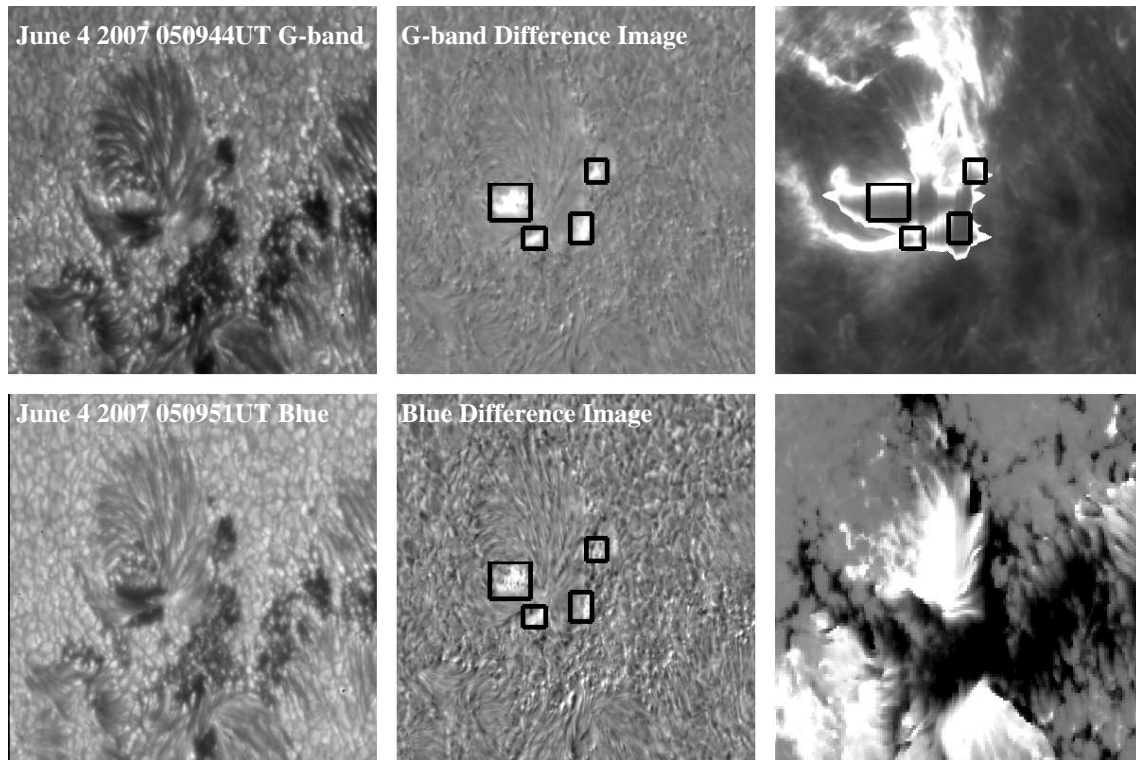
Fig. 1 Comparison of white-light emissions in the G-band and blue continuum of the M8.7 flare on 2007 June 4. Top panels: pre-flare image in G-band, difference image at the peak of the flare and corresponding image in CaII H band. Bottom panels: pre-flare image in blue continuum, difference image at the peak of the flare and the corresponding line-of-sight magnetogram obtained at 12UT. Four flare kernels are marked by dark boxes. The flare images were obtained at 051243UT and 051249UT for the G-band and blue continuum, respectively, while the pre-flare images were at 050944UT and 050951UT. The field-of-view is 43.6 by 43.6 arcsec.
