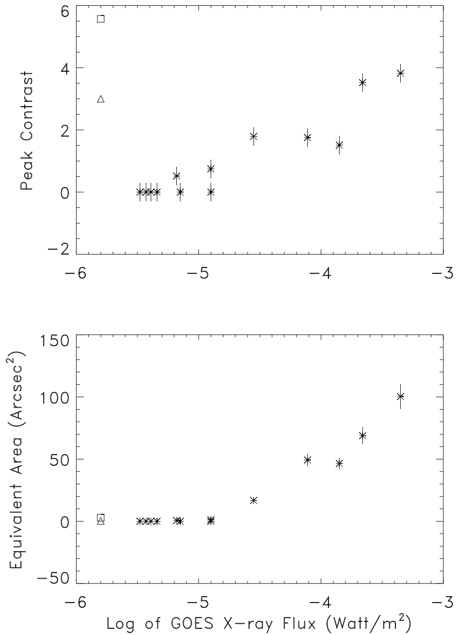
Fig. 2 The correlation between GOES X-ray flux and the flare emission in G-band. The top panel plots the peak contrast while the bottom panel plots the equivalent area. The triangles and squares mark the corresponding emission of the C2.0 flare of 2007 August 24 observed by Jess et al. (2008) for the blue continuum and extrapolated G-band emissions. The values of -6, -5 and -4 in X-axis mark the beginning of C, M, and X-class flares.
